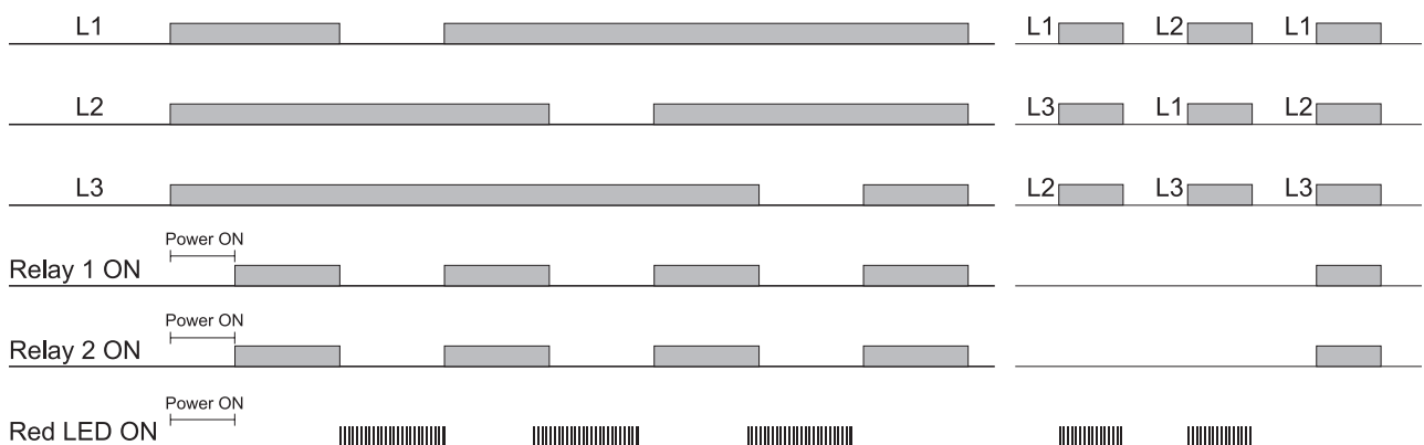
Fig. 4 Phase sequence, total phase loss
